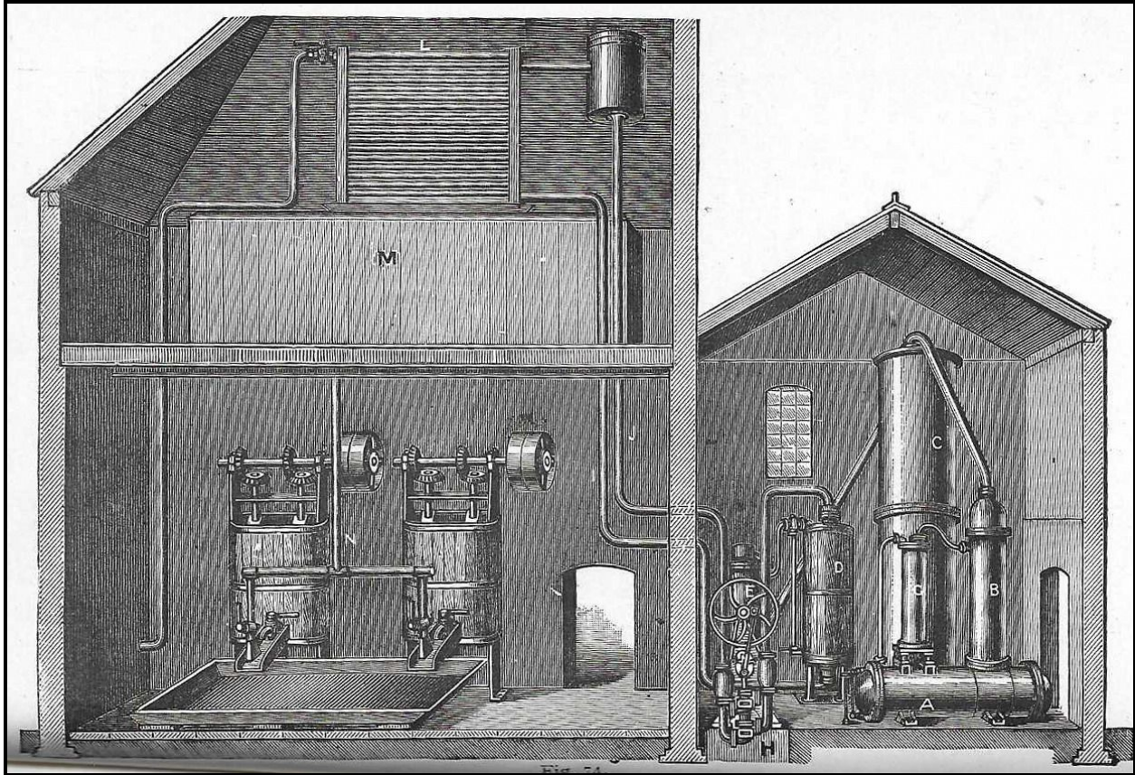
Ammonia Absorption Machine
