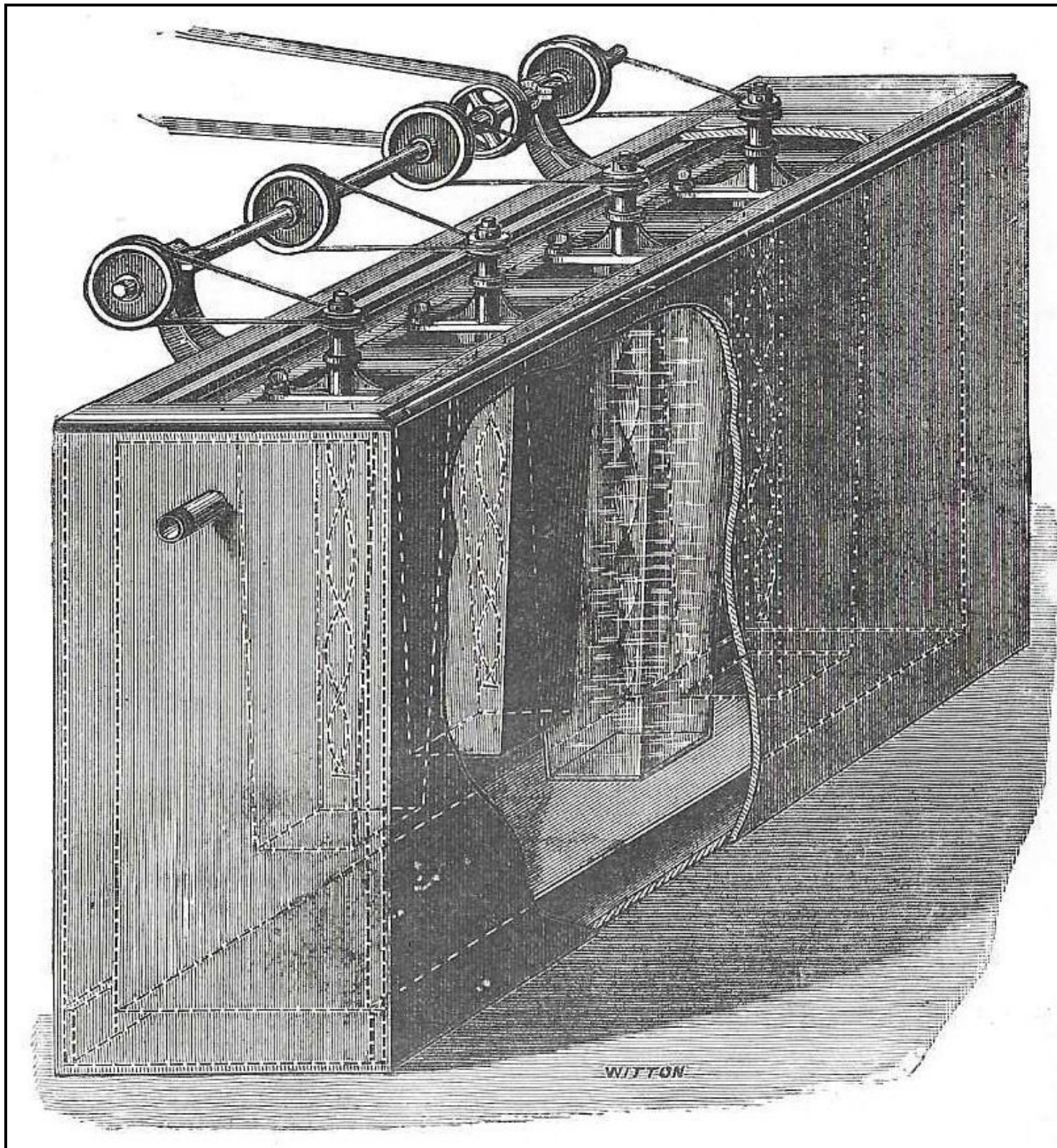
Ice-Making Tank with Internally Cooled Chambers
