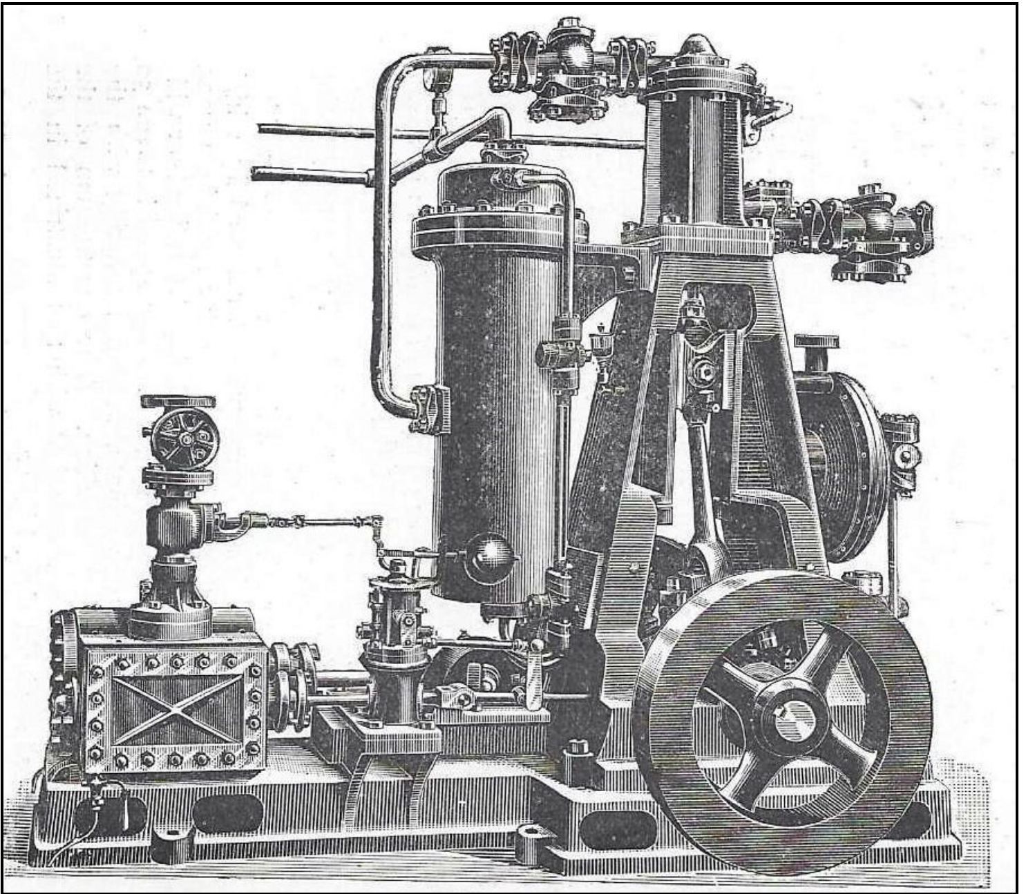
Ammonia Refrigerating Plant
