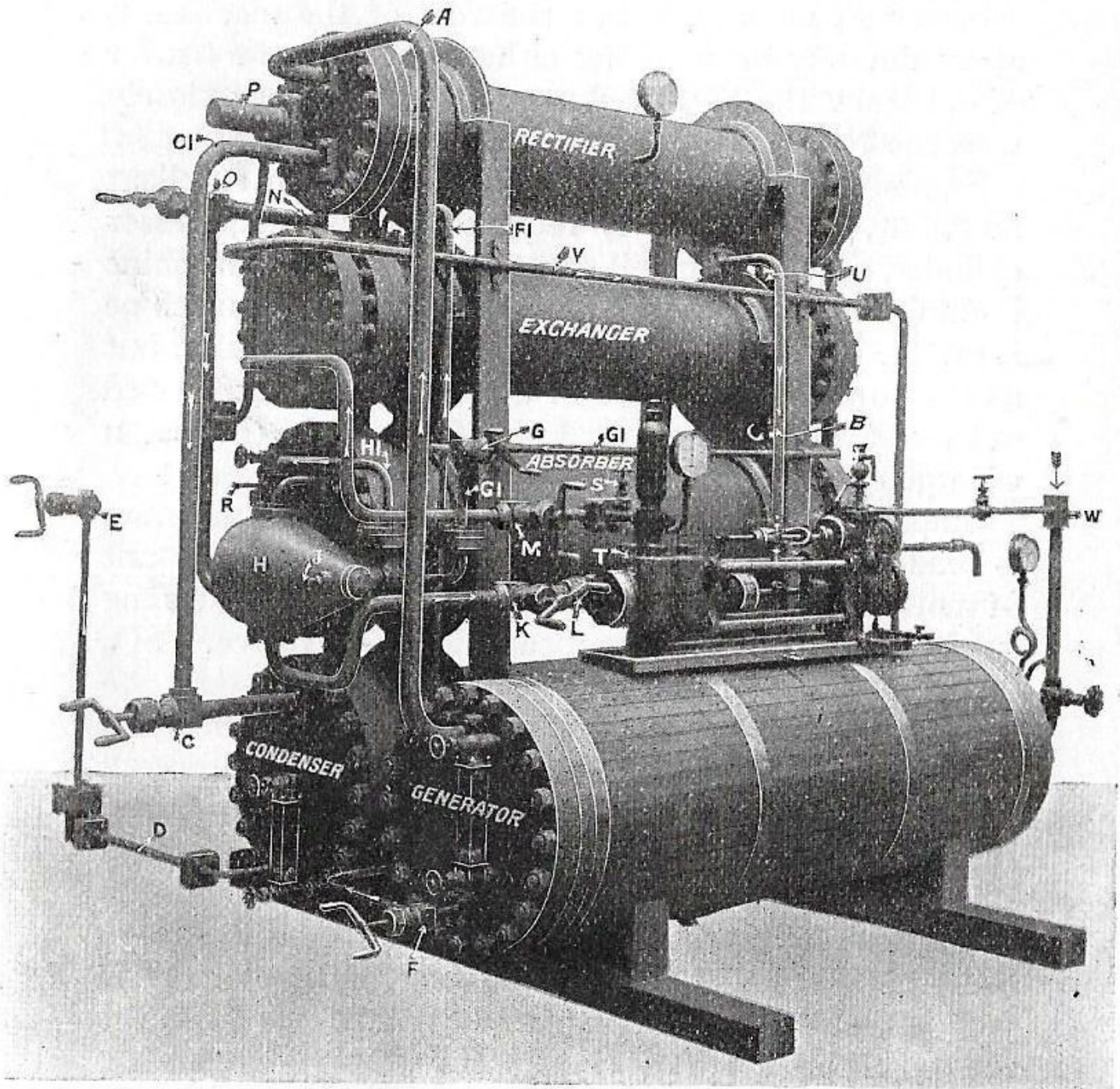
FIG. 9 ABSORPTION REFRIGERATING MACHINE BY MESSRS. RANSOMES & RAPIER, LTD.
