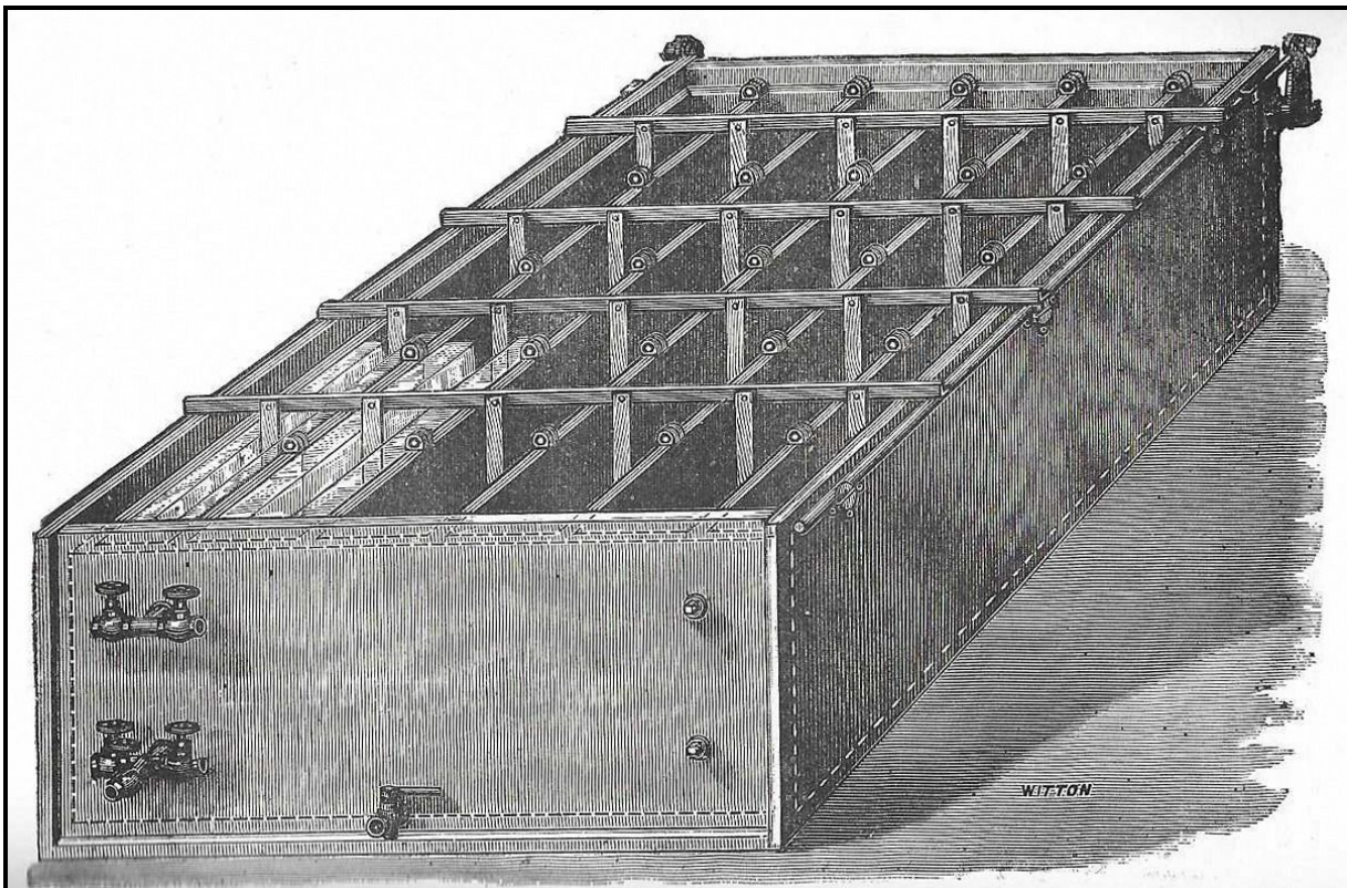
Ice-Making Tank with Rotary Agitators
