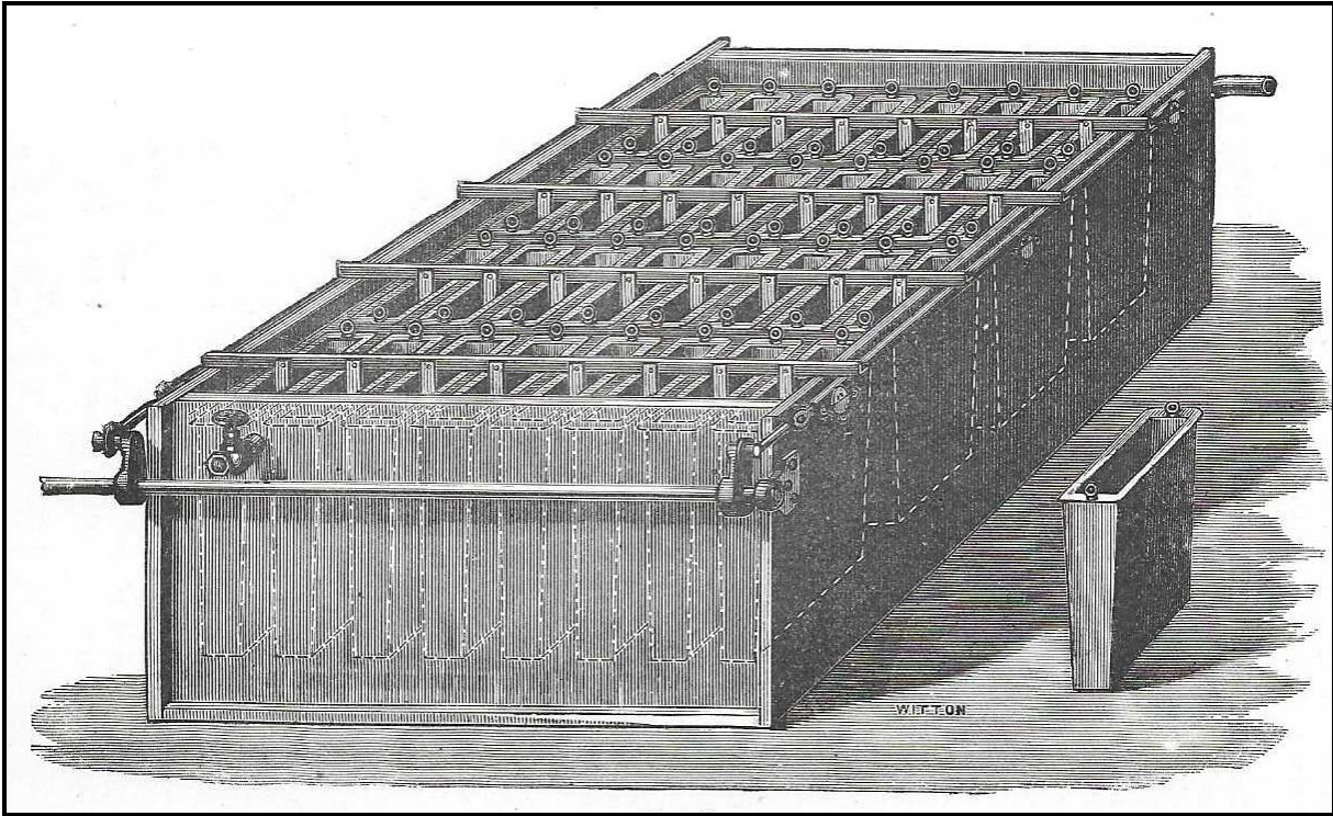
Ice-Making Tank with Rotary Agitators
